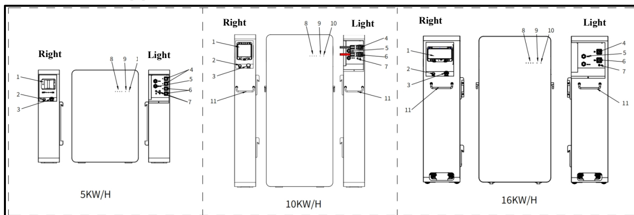
Figure 2-3 Battery Appearance
