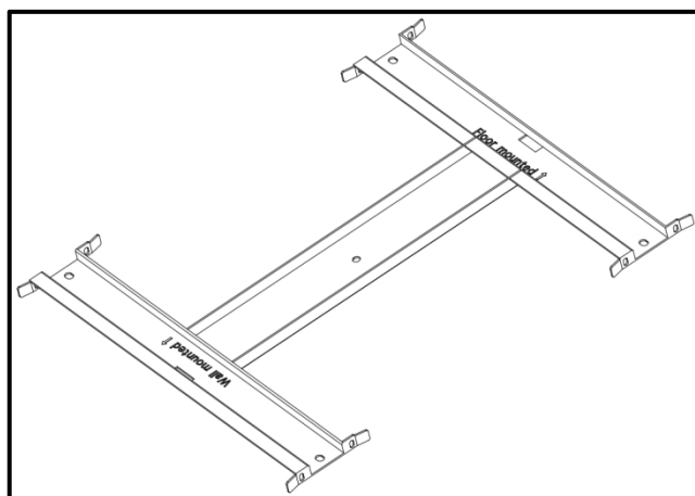
Figure 4.3 Wall mounted bracket for IntelliHome 14kWh&16kWh (Optional accessory)
