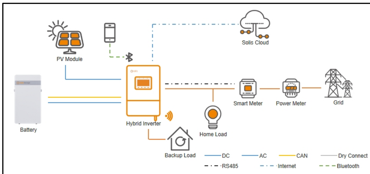
Figure 2-4 System Diagram
