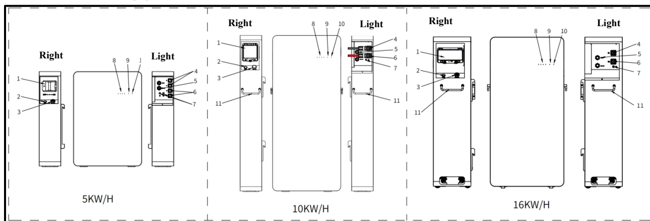
Figure 2-3 Battery Appearance
